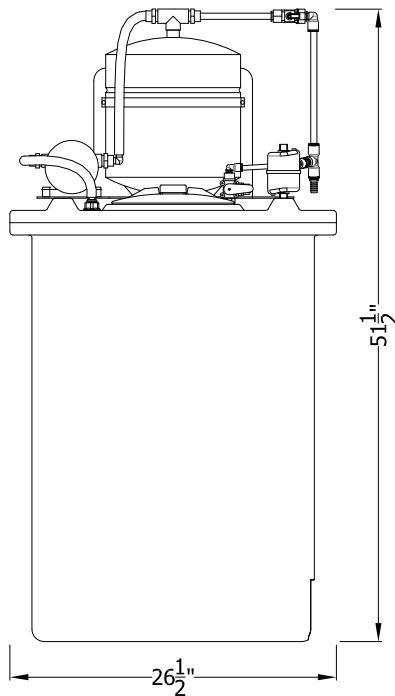
Repressurization/Storage Tank Assembly
